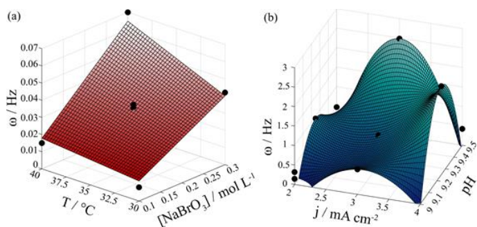
Figure 1. Surfaces responses (a) Chemical Oscillator (BZ reaction) and (b) Electrochemical Oscillator (Cu/Cu 2 O - Cathodic Deposition).
