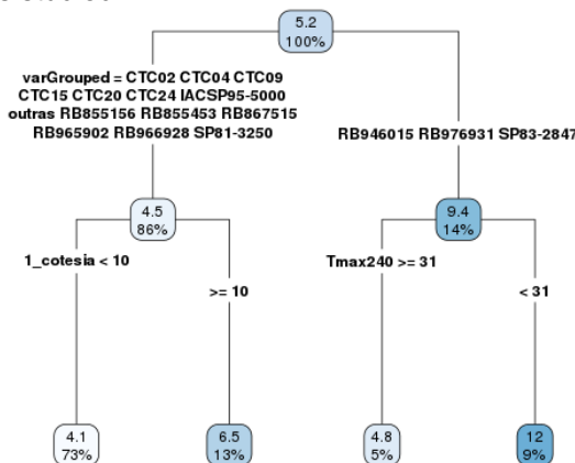
Image 1. Regression tree with better metrics among the 60 models studied.
